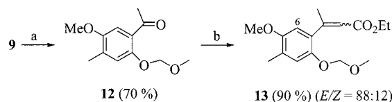
Scheme 2. a) \text{ClCH}_2\text{OCH}_3 , i\text{Pr}_2\text{Net} , \text{CH}_2\text{Cl}_2 , room temp. b) (\text{EtO})_2\text{P}(\text{O})\text{CH}_2\text{CO}_2\text{Et} , NaH, THF, reflux.
