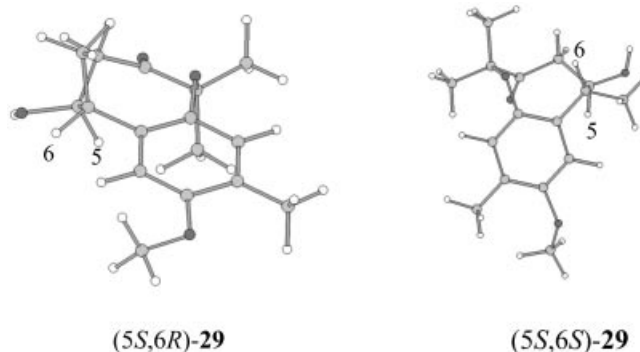
Figure 7. PM3-minimized geometries of ( 5S,6R )- and ( 5S,6S )- 29 .
