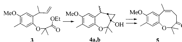
Figure 2. Synthesis of potential precursor 5 .
